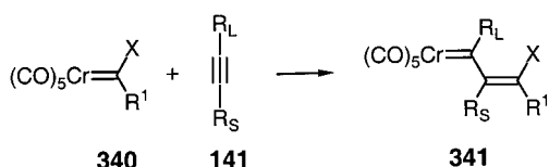
Scheme 30. R_L = larger, R_S = smaller substituent; X = OR, NR 2 .
